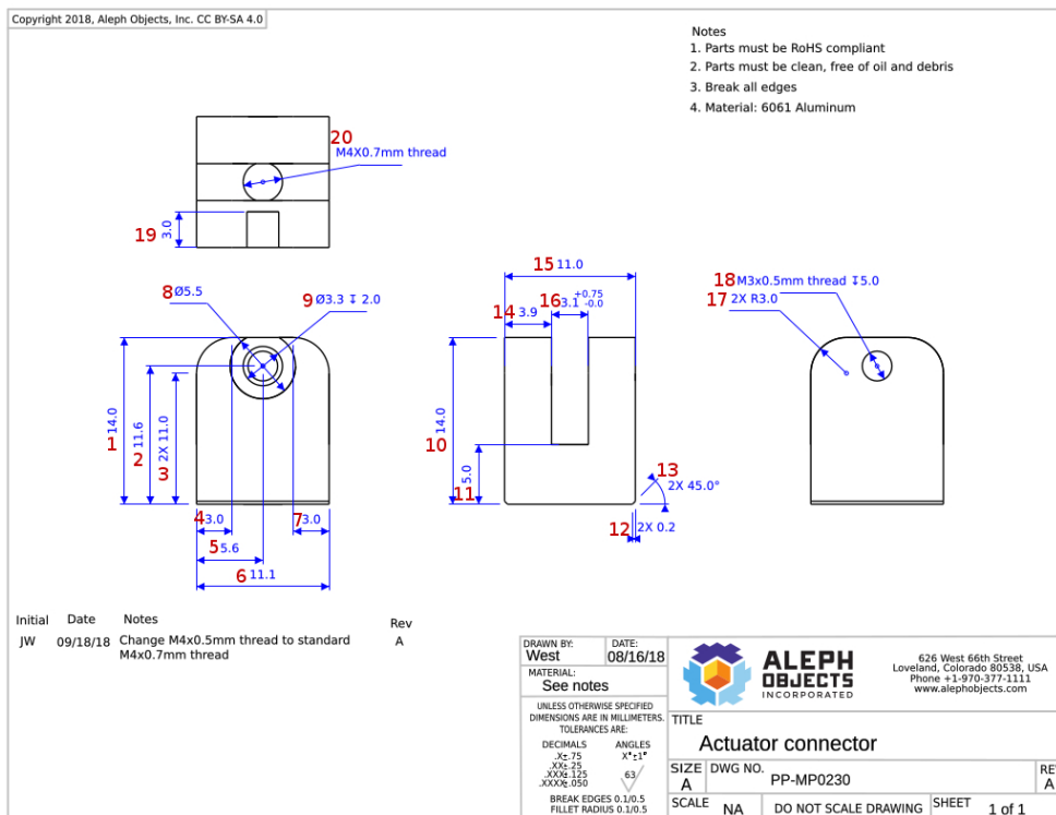
Figure 1: Schematic of PP-MP0230.
