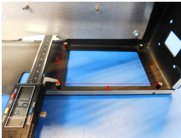
Figure 4: Dimensions of Drawing 2.
