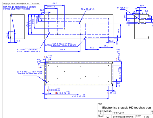
Figure 1: Schematic 01 of PP-FP0149.
