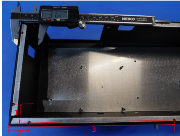
Figure 3: Dimensions of Drawing 1.
