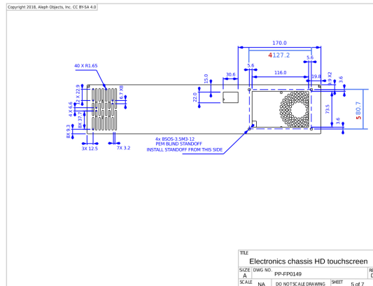
Figure 2: Schematic 02 of PP-FP0149.
