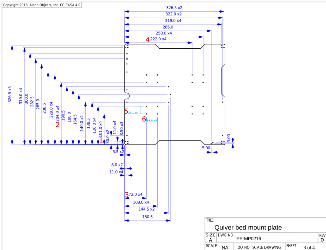
Figure 1: Schematic of PP-MP0216.
