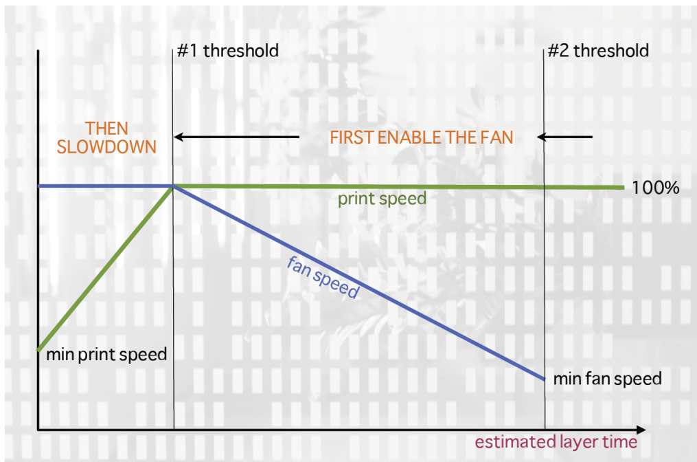
Figure 2.35: Cooling strategy.
