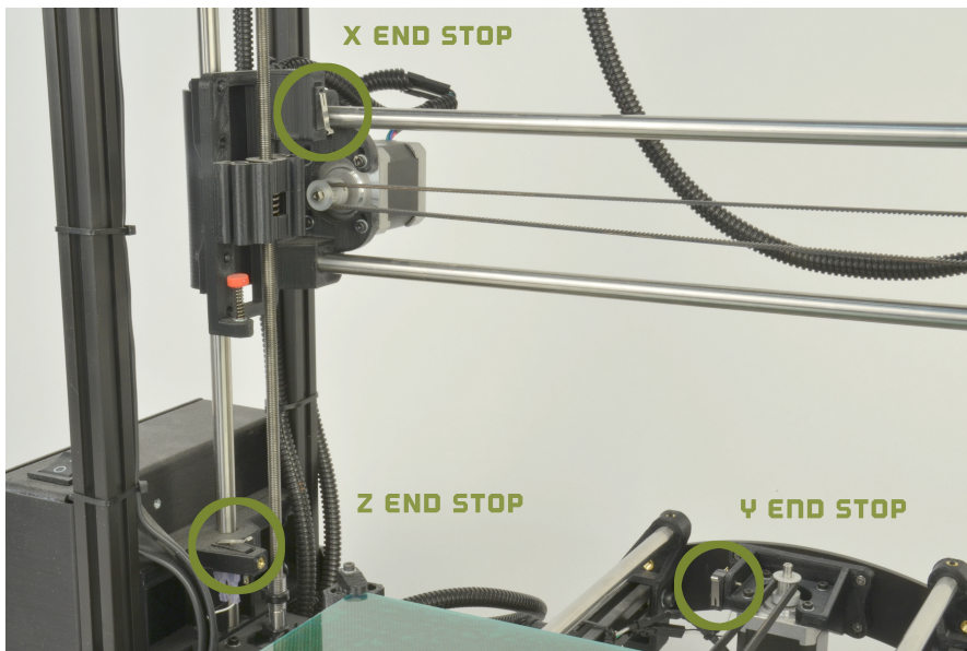
Figure 1.22: End stop locations
