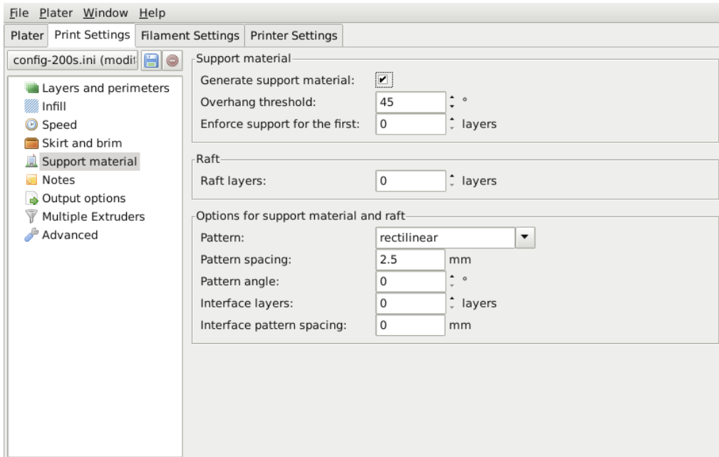
Figure 5.37: Support structure options.
