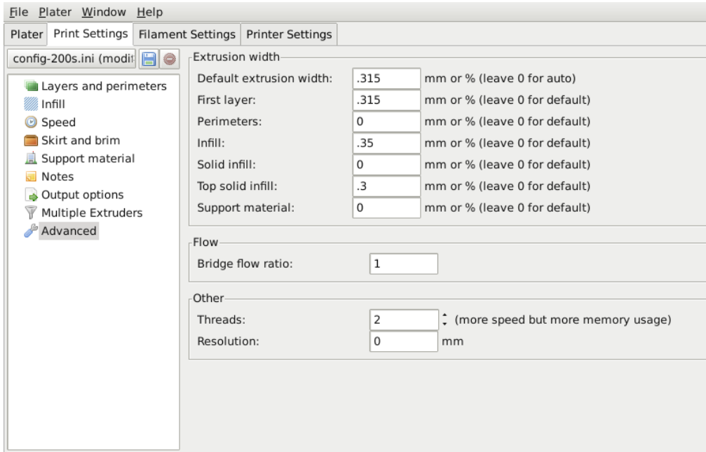
Figure 5.48: Extrusion widths options.
