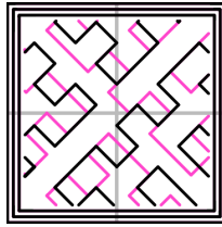
Figure 5.27: Infill pattern: Hilbert Curve (332.82mm / 5m:28s)
