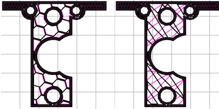
Figure 5.30: Infill pattern comparison in a complex object. Left to Right: honeycomb, line
