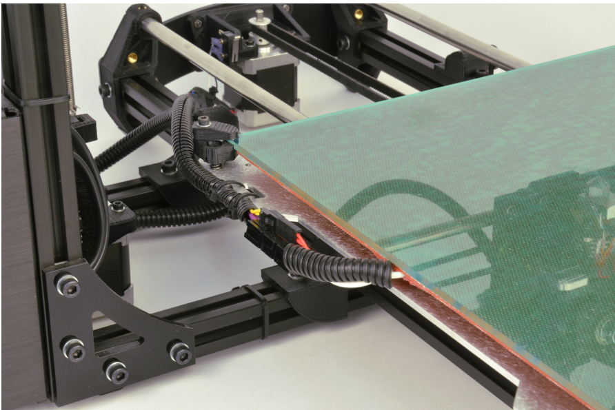
Figure 1.10: Tightly wrap the zip ties around the bed wires and through the strain relief slot
