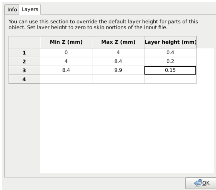
Figure 5.52: Variable layer height options - Layers.
