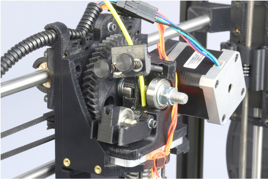
Figure 4.4: Extruder filament slot
