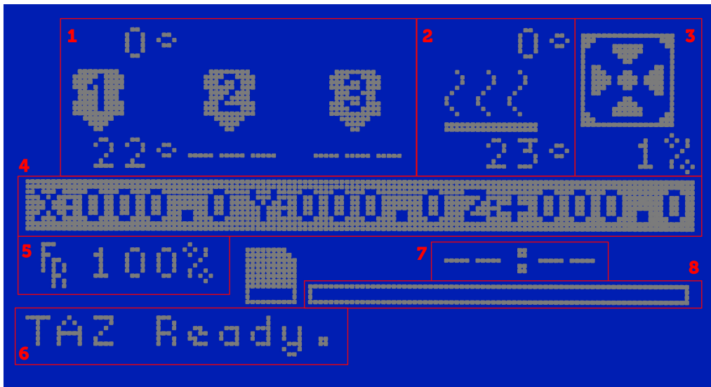
Figure 6.1: GLCD Info Screen
