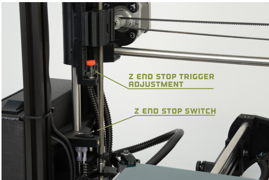
Figure 4.6: Z end stop trigger
