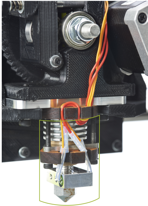
Figure 5.60: The clearance cylinder around an extruder.
