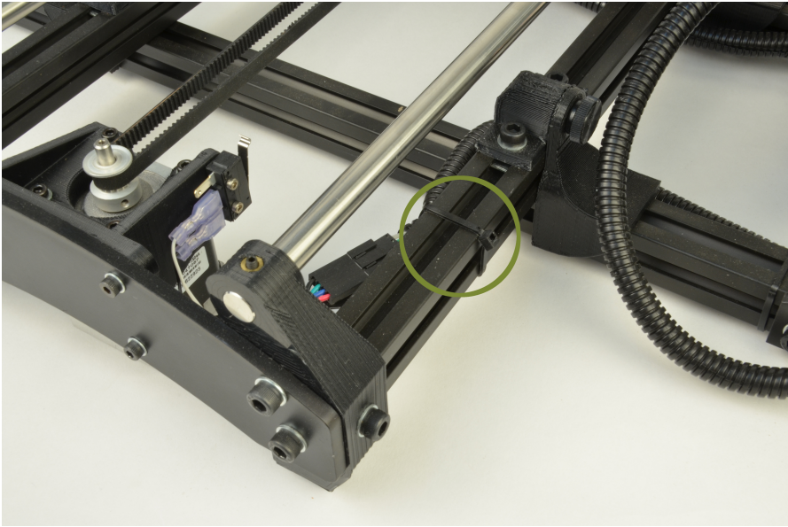
Figure 1.7: Wrap and tighten a zip tie around the Y axis wires to the Y axis frame.
