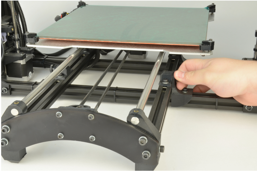
Figure 1.5: Screw in and tighten the four Y axis bolts
