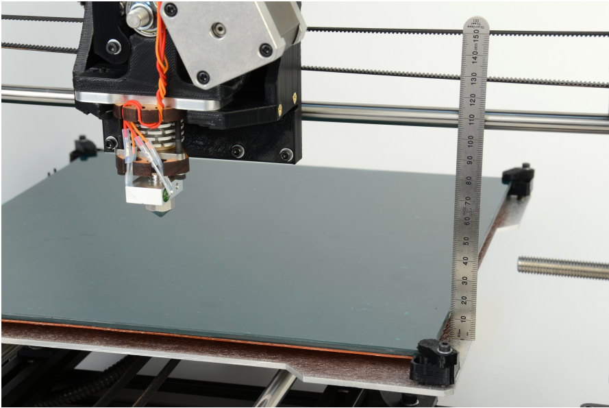
Figure 4.2: Verifying the X and Y axis are square
