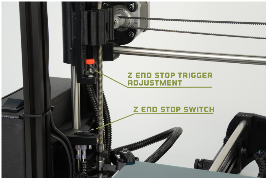
Figure 4.1: Z end stop trigger
