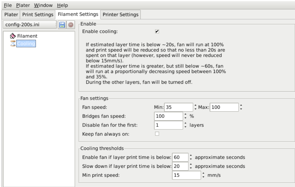
Figure 5.36: Cooling advanced settings.
