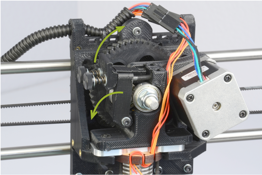
Figure 4.3: Extruder idler release
