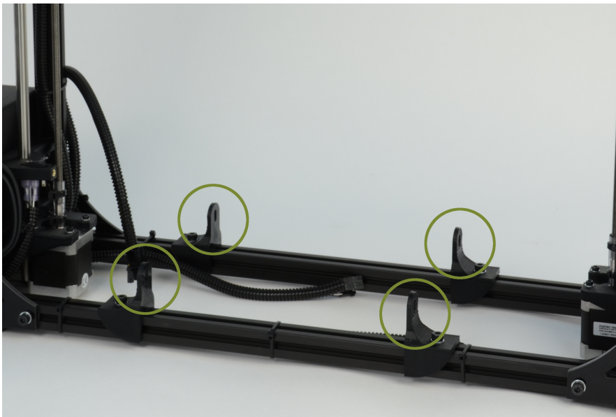
Figure 1.4: Locate the four Y axis mounts on the frame
