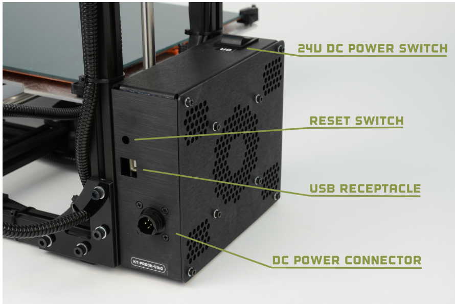
Figure 1.14: Power and USB receptacles
