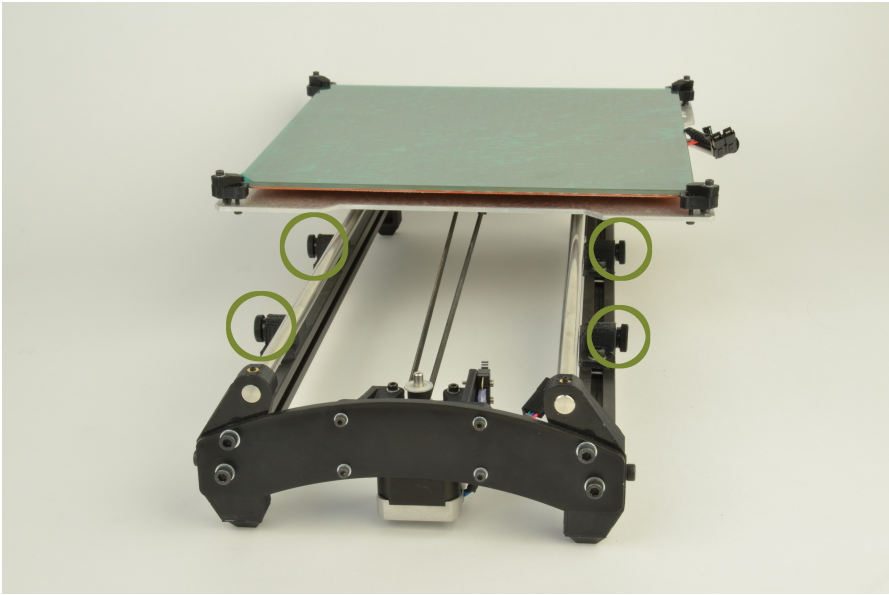
Figure 1.2: Locate the four Y axis bolts
