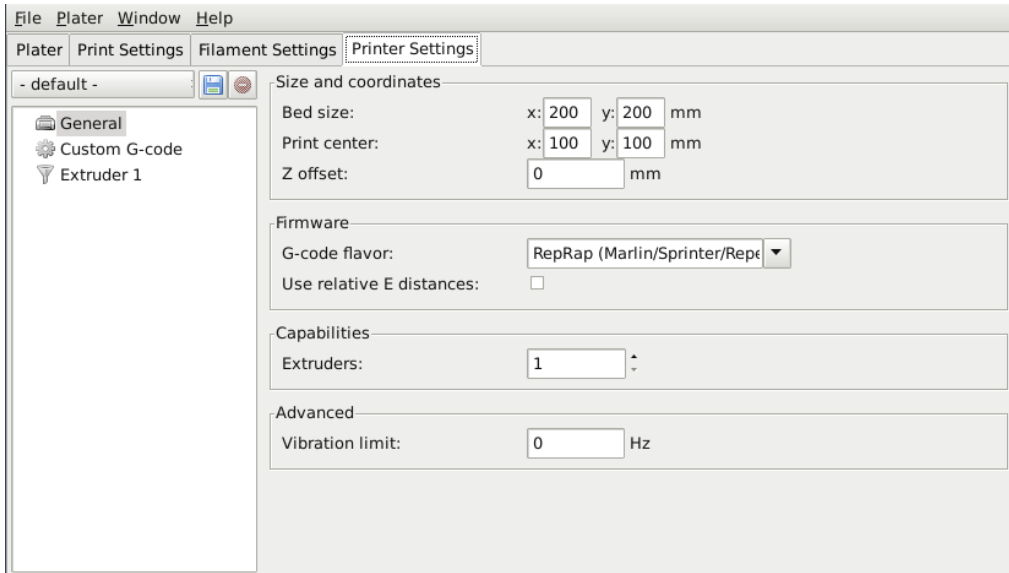
Figure 5.43: Multiple extruder options - Printer Settings Tab (General). Note the two extruders defined in the left-hand pane.
