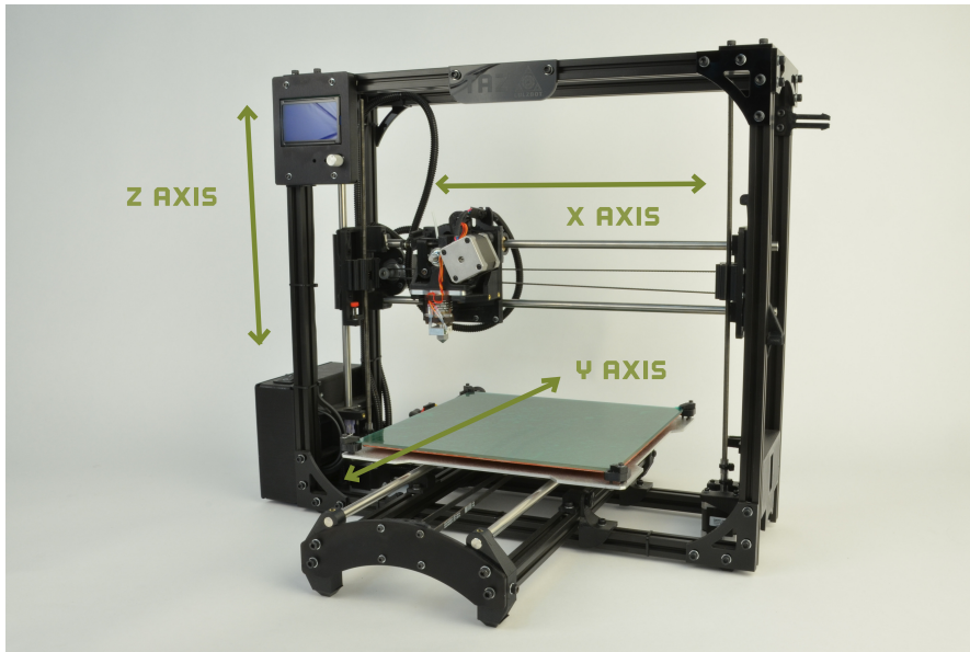
Figure 1.21: Axes movement directions
