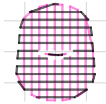
Figure 5.40: Support infill pattern: Rectilinear Grid
