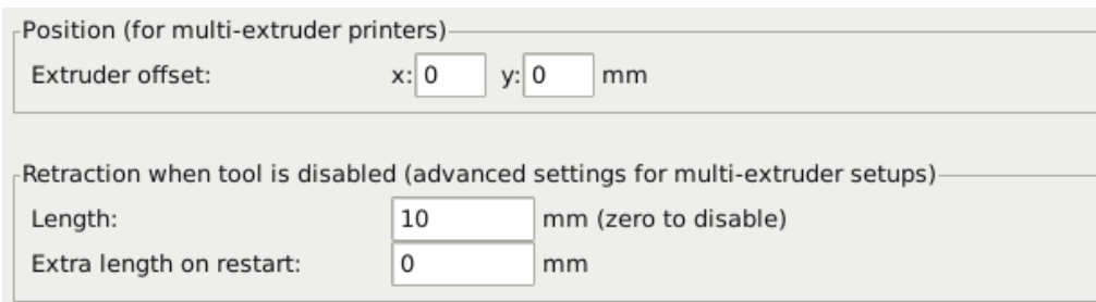
Figure 5.44: Multiple extruder options - Printer Settings Tab (Extruder).
