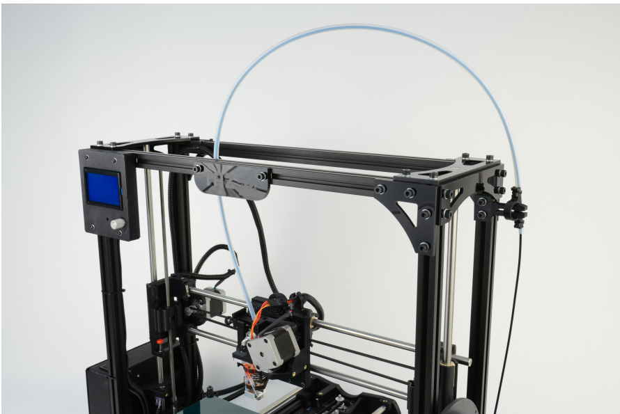
Figure 1.20: Filament Guide Setting
