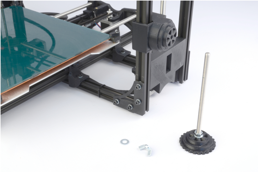
Figure 2.1: Filament spool mount parts
