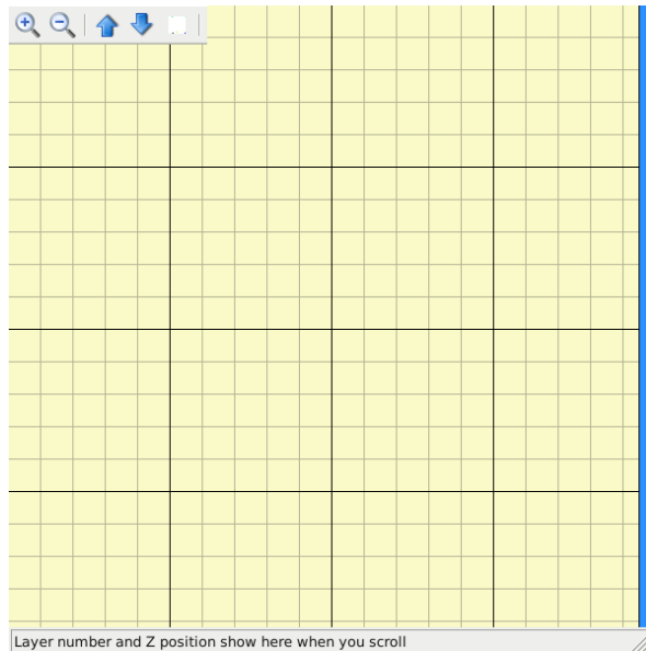
Figure 2.4: Printrun viewer
