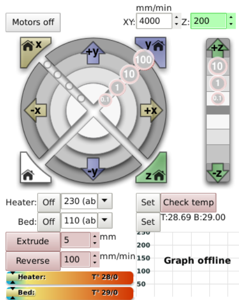
Figure 2.3: Printrun controls
