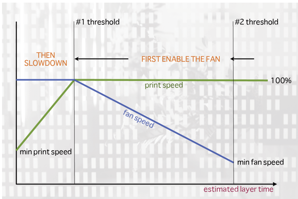
Figure 3.34: Cooling strategy.
