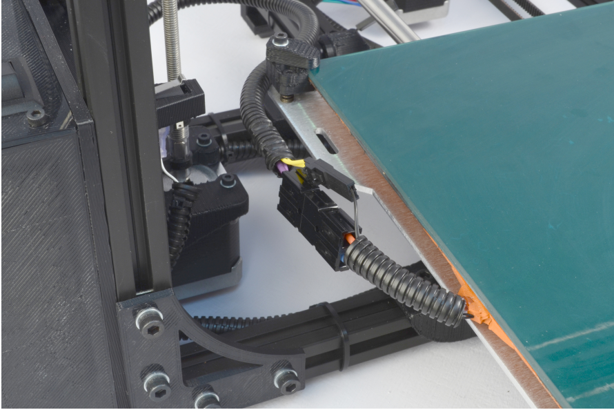
Figure 1.6: Connect the two connectors on the left of the print bed
