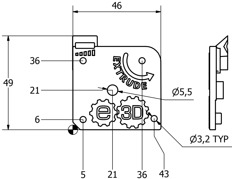
TITAN-LID-RH
