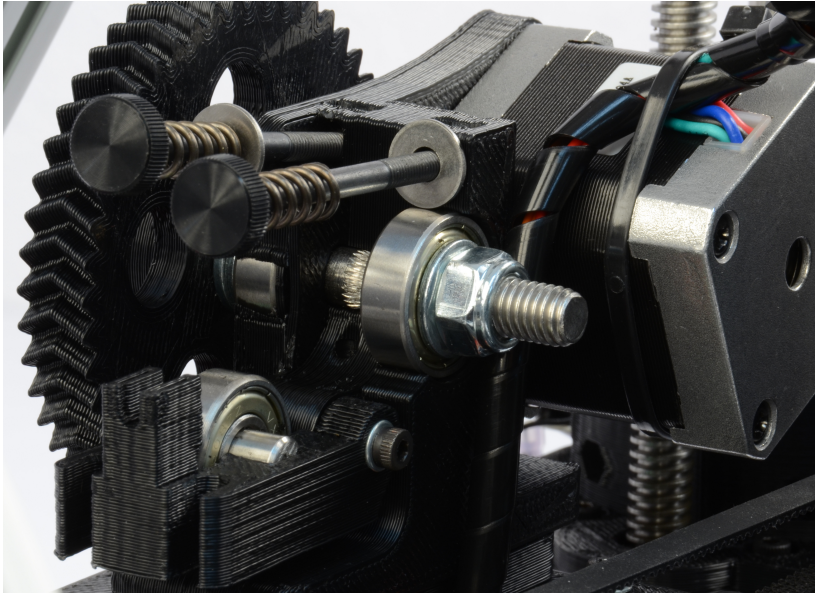
Figure 5.2: Extruder feed hole
