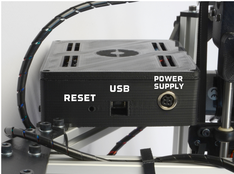
Figure 2.4: Power supply and USB receptacles
