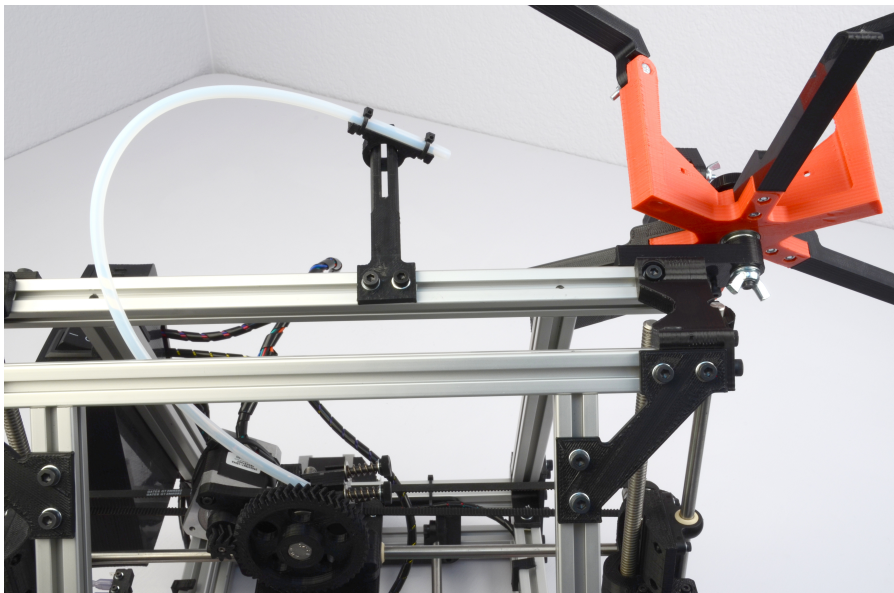
Figure 2.12: Filament Guide Setting
