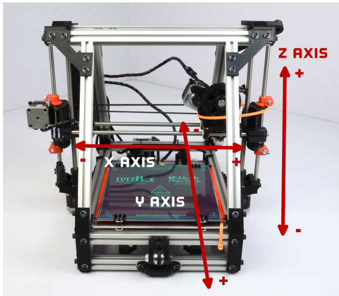
Figure 2.1: Axes movement directions
