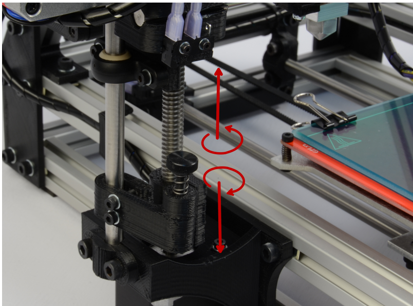
Figure 5.4: Z endstop trigger
