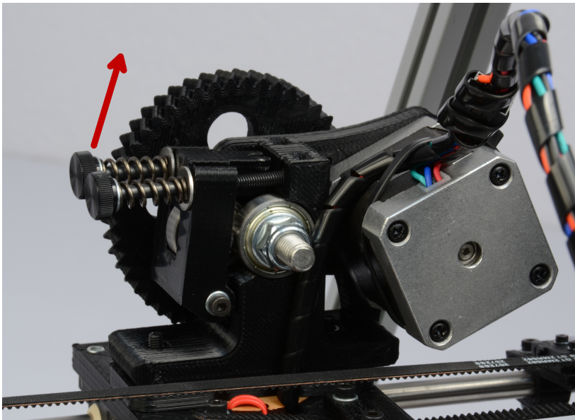
Figure 5.1: Extruder idler bolts
